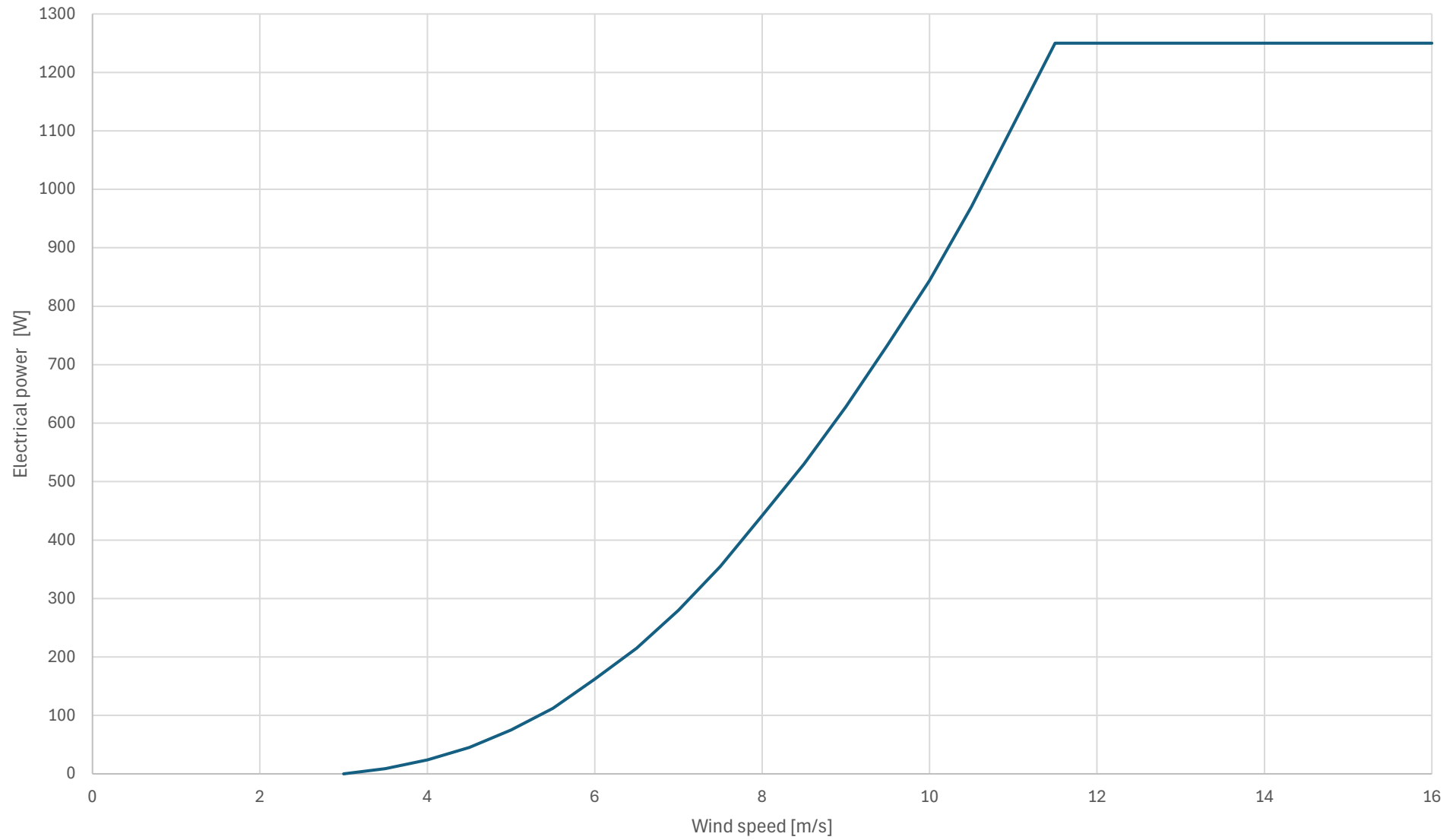
SW 1250 Power curve
